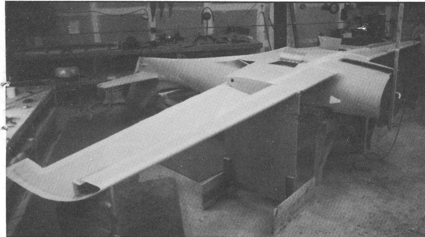
Wing assembly requires only two cradles.
